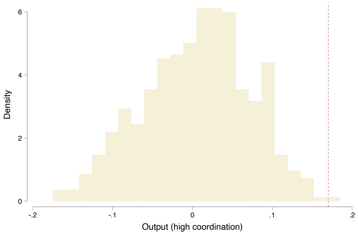
Figure C.3: RI estimates of treatment effects on output (high coordination teams)
