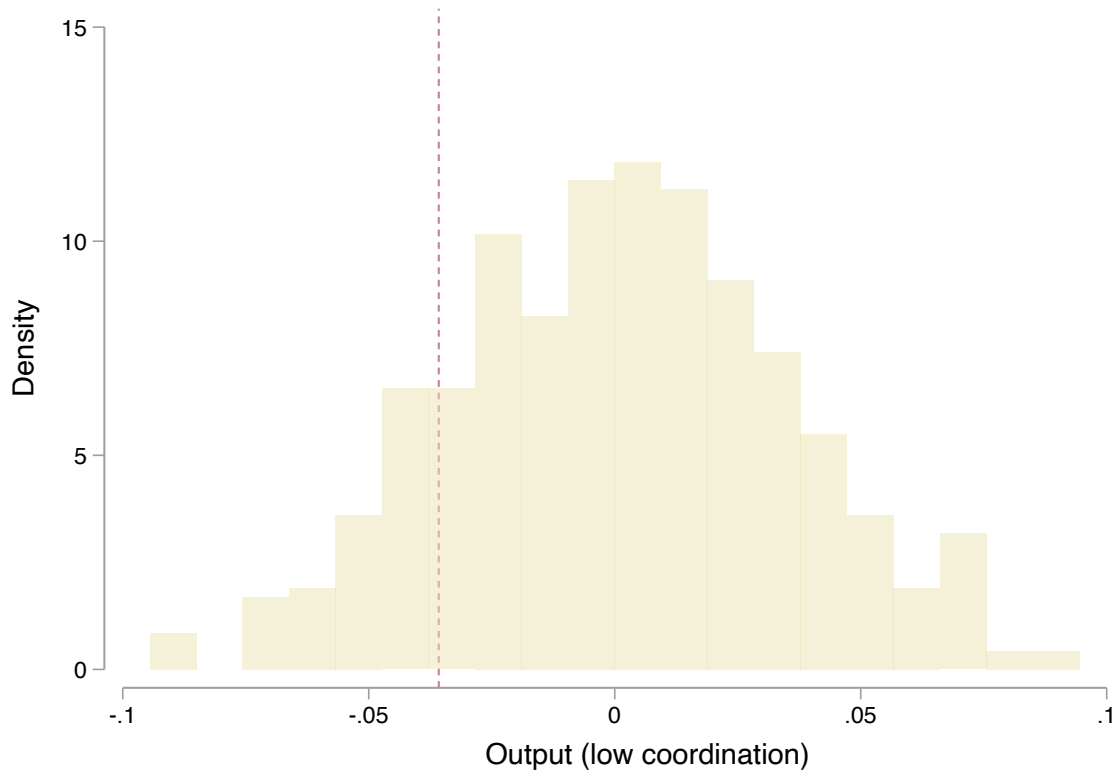
Figure C.2: RI estimates of treatment effects on output (low coordination teams)
